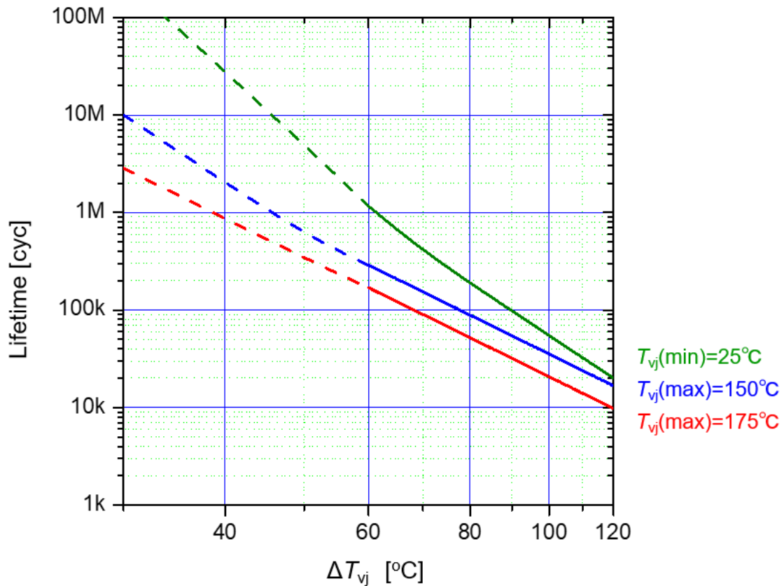
Typical \Delta T_{vj} Power cycling lifetime curve I_C \leq I_{C(rated)} , F(t)=1\%
